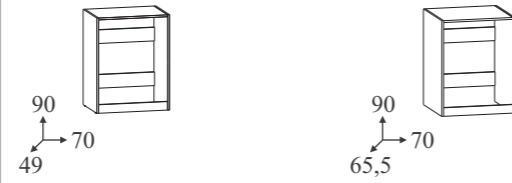
Pensile / Wall-mounted unit Hängeschrank Armoire suspendue
